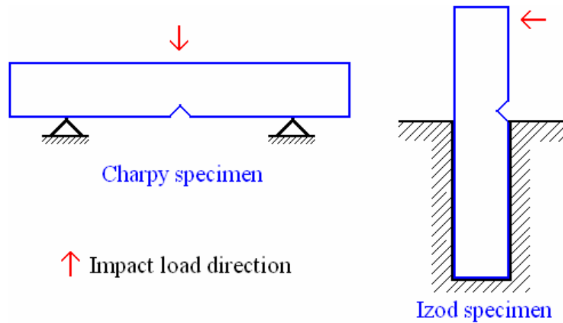
Figure-4: Loading of Charpy and Izod notched-bar impact testing specimens.
