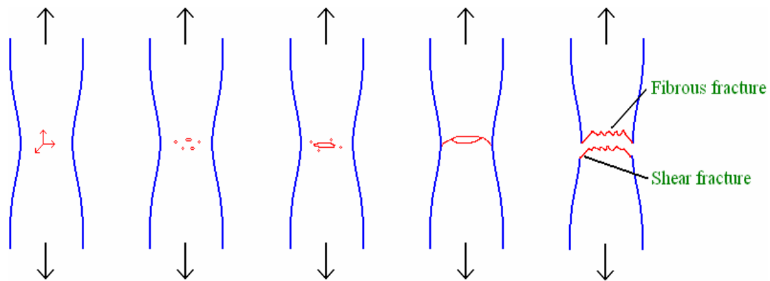
Figure-2: Stages of ductile tensile fracture- void nucleation, void growth, crack initiation and eventual fracture under ductile fracture mode
