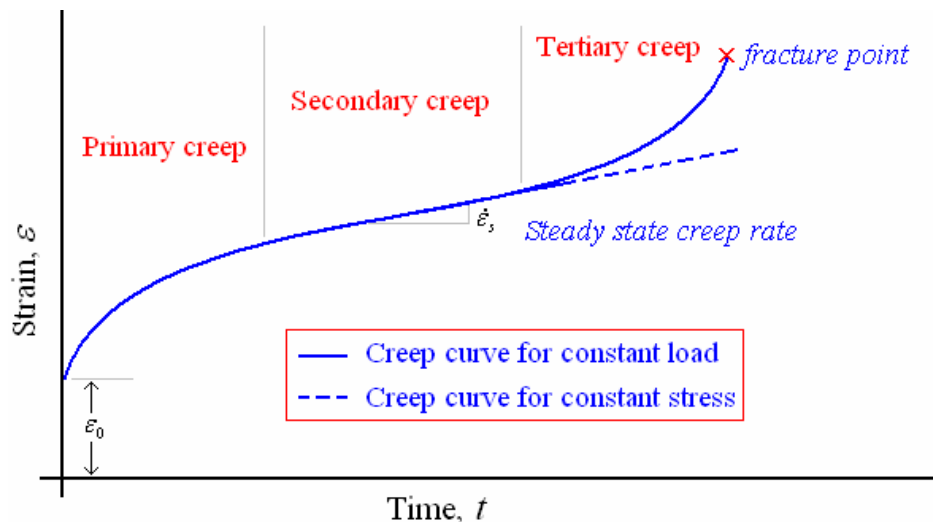
Figure-8: Typical creep curve
