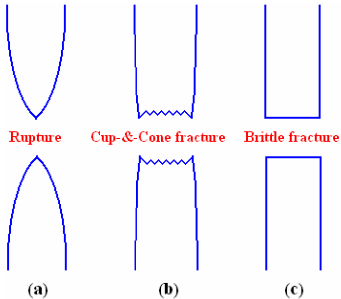
Figure-1: Types of fractures observed in metals subjected to uniaxial tension (a) completely ductile fracture in polycrystals (b) ductile fracture in polycrystals (c) brittle fracture of single crystals and polycrystals.
