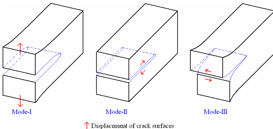
Figure-3: Crack deformation modes.
